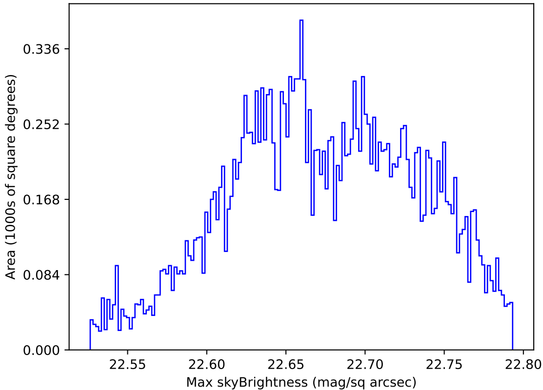
ddf_acor_sf20_lsf0_lsr0_v3.4_10yrs Yr 1 u band: Max skyBrightness
