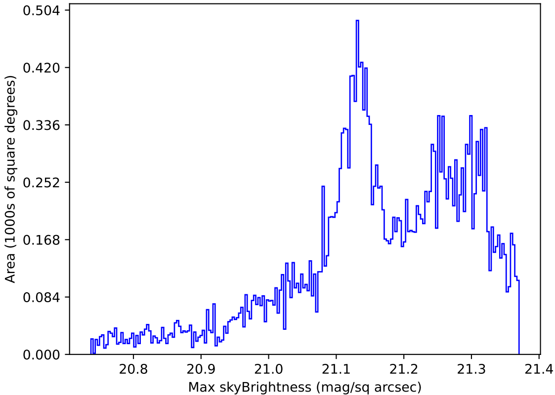
ddf_acor_sf20_lsf0_lsr0_v3.4_10yrs Yr 1 r band: Max skyBrightness
