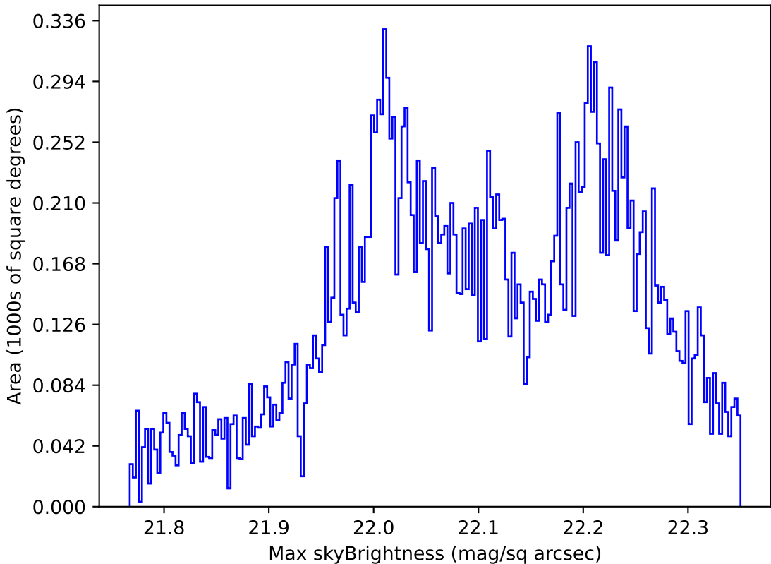
ddf_acor_sf20_ls0_lsr0_v3.4_10yrs Yr 1 g band: Max skyBrightness
