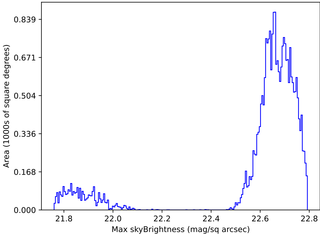
ddf_acor_sf20_lsf0_lsr0_v3.4_10yrs Yr 1 all bands: Max skyBrightness
