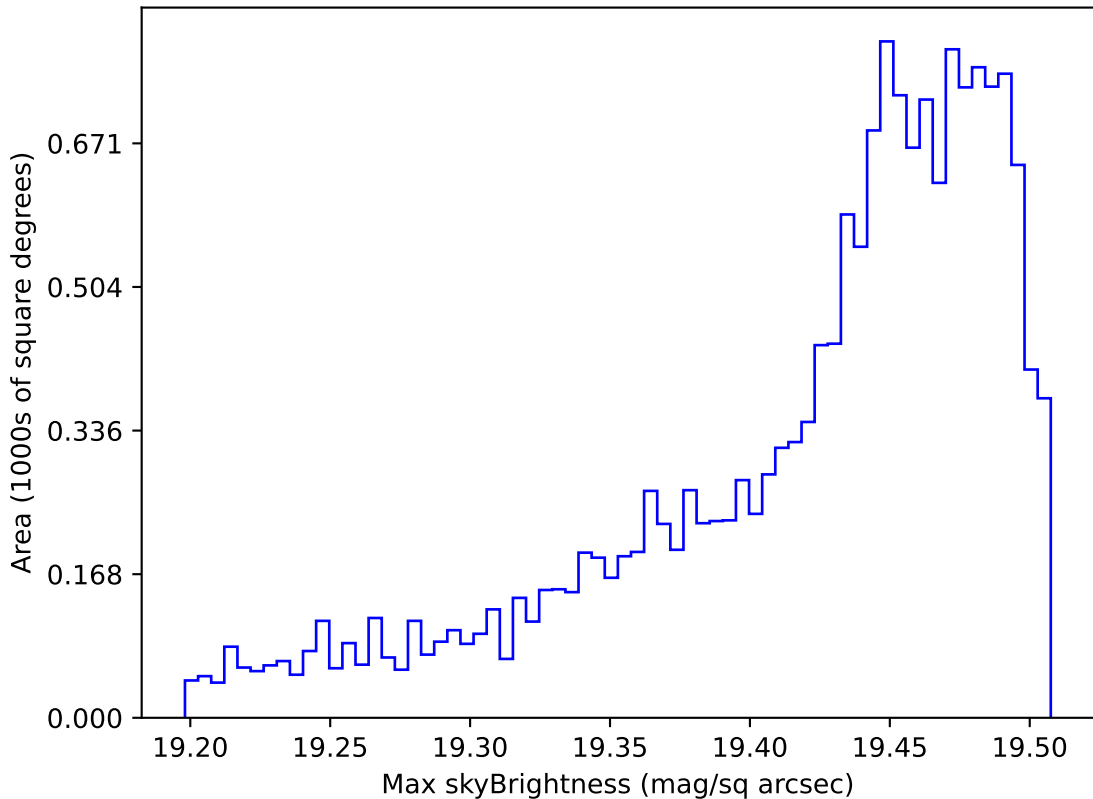
ddf_acor_sf20_ls0_lsr0_v3.4_10yrs WFD z band: Max skyBrightness
