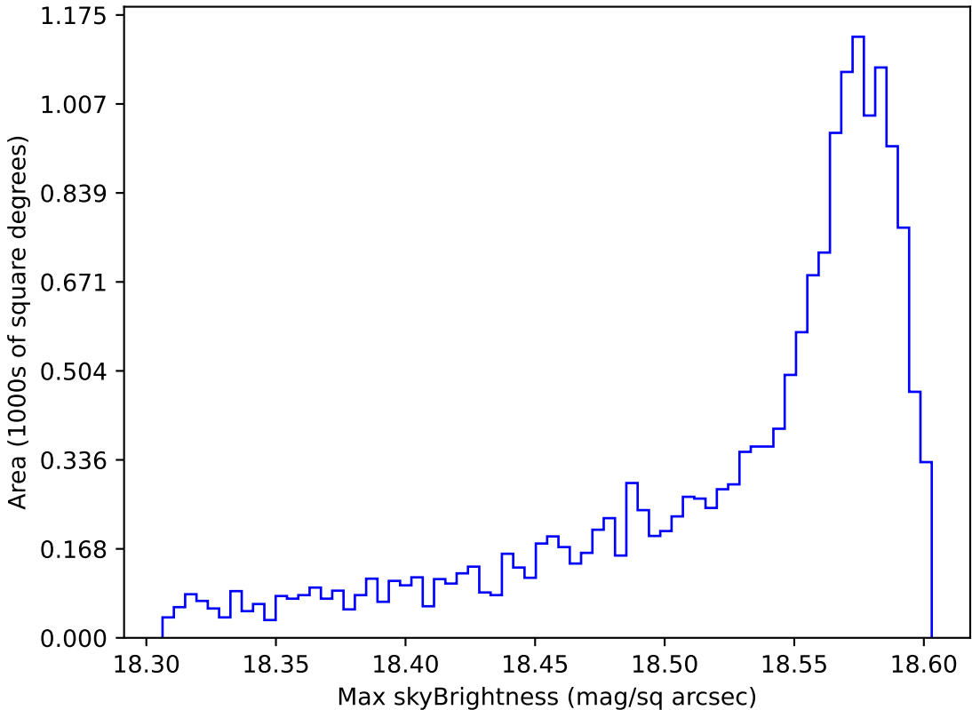
ddf_acor_sf20_lsf0_lsr0_v3.4_10yrs WFD y band: Max skyBrightness
