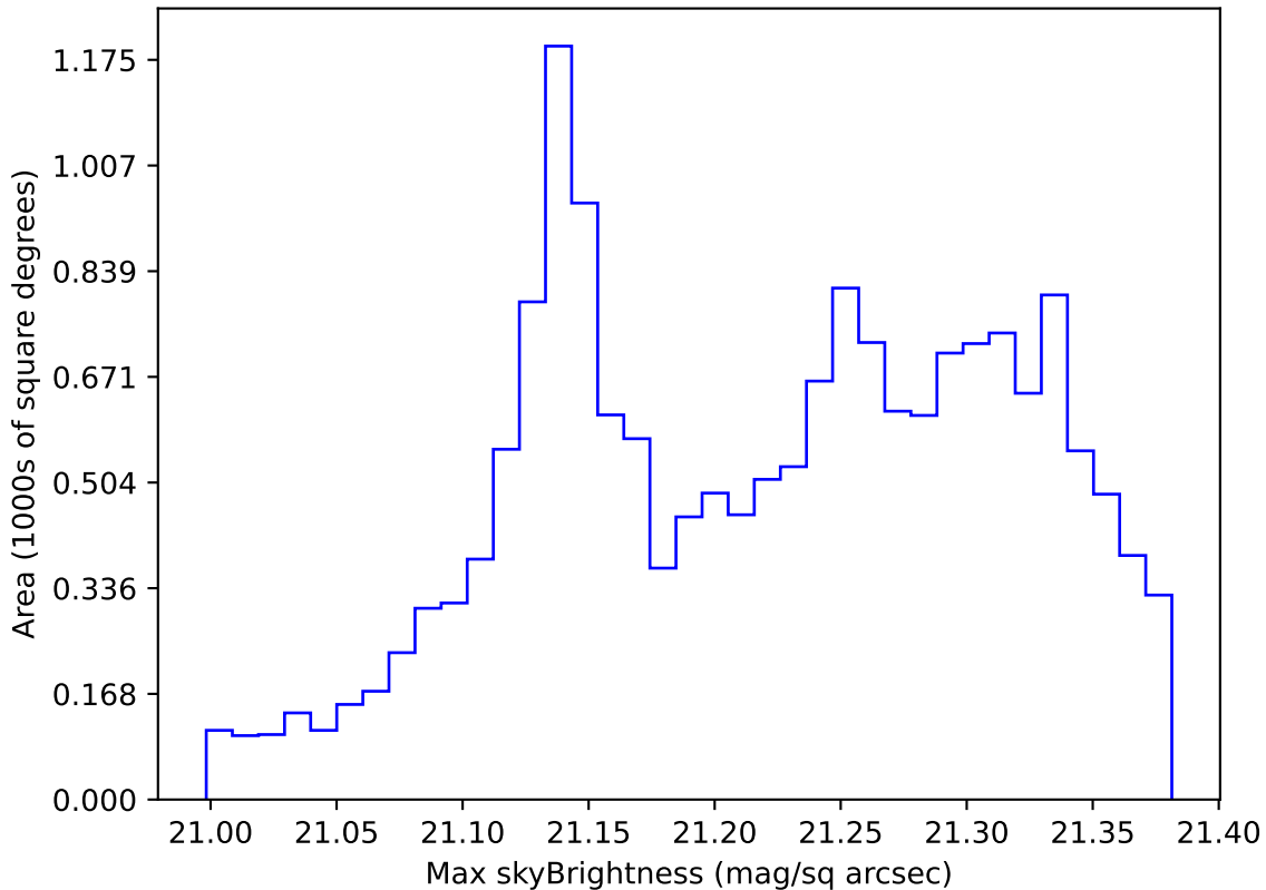
ddf_acor_sf20_lsf0_lsr0_v3.4_10yrs WFD r band: Max skyBrightness
