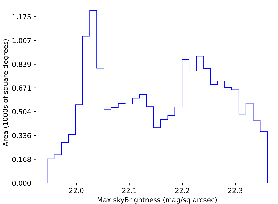
ddf_acor_sf20_ls0_ls0_v3.4_10yrs WFD g band: Max skyBrightness
