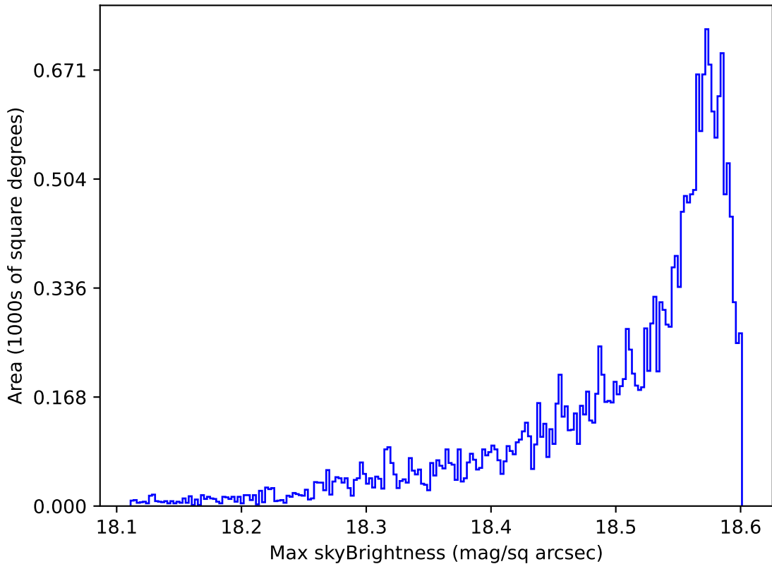
ddf_acor_sf20_lsf0_lsr0_v3.4_10yrs All sky y band: Max skyBrightness
