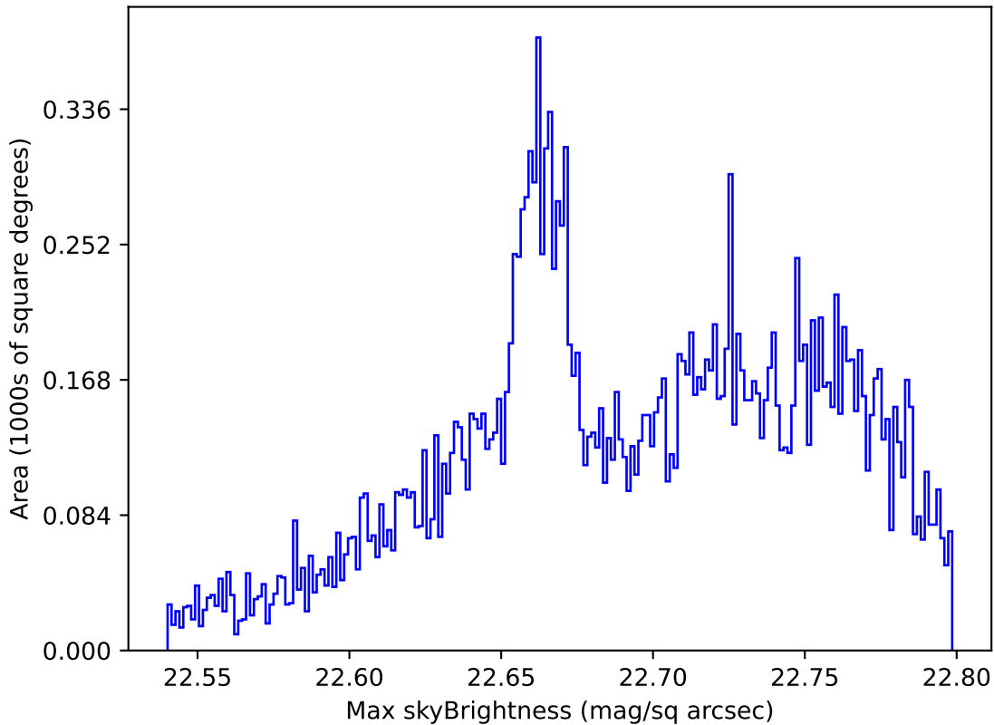
ddf_acor_sf20_lsf0_lsr0_v3.4_10yrs All sky u band: Max skyBrightness
