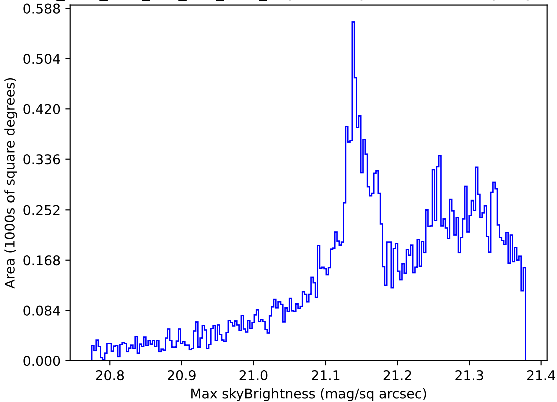
ddf_acor_sf20_lsf0_lsr0_v3.4_10yrs All sky r band: Max skyBrightness
