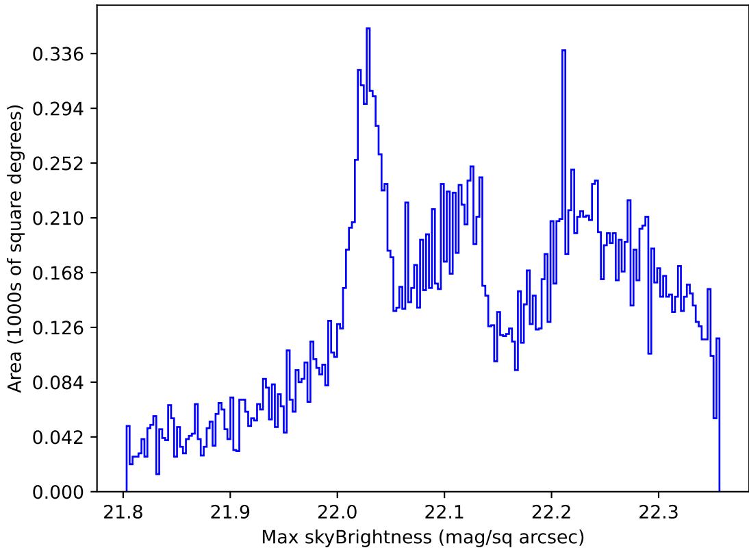
ddf_acor_sf20_lsf0_lsr0_v3.4_10yrs All sky g band: Max skyBrightness
