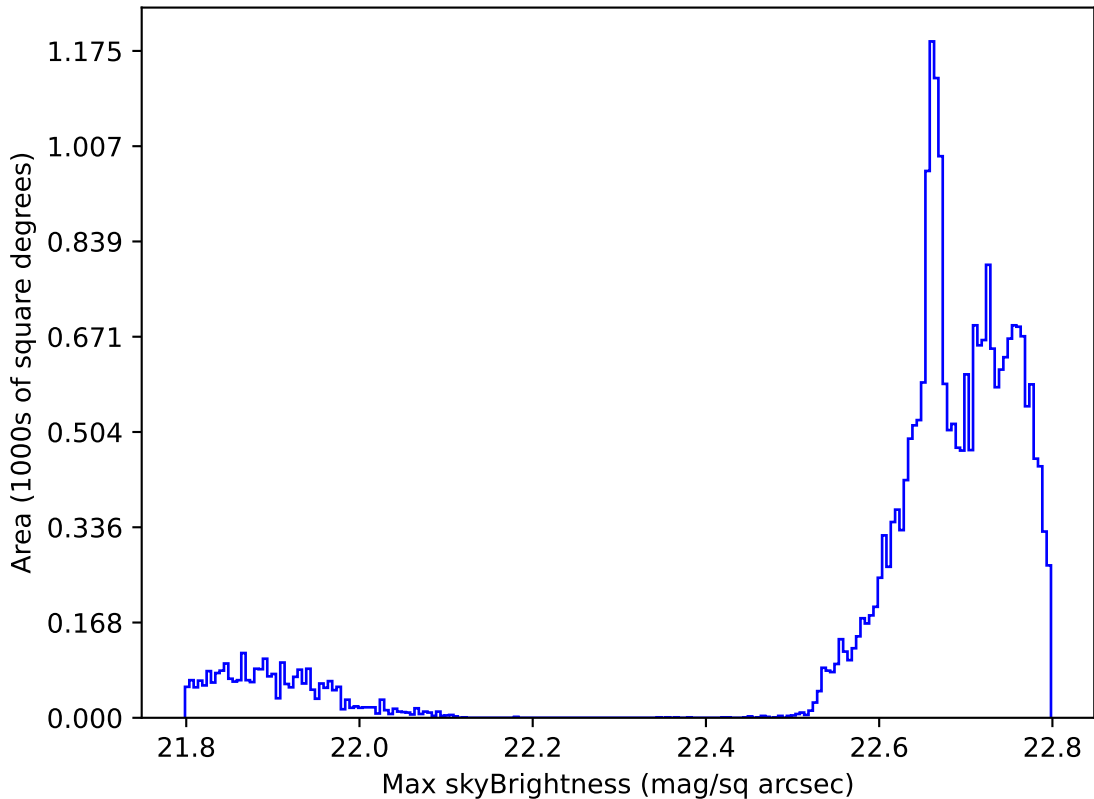
ddf_acor_sf20_lsf0_lsr0_v3.4_10yrs All sky all bands: Max skyBrightness
