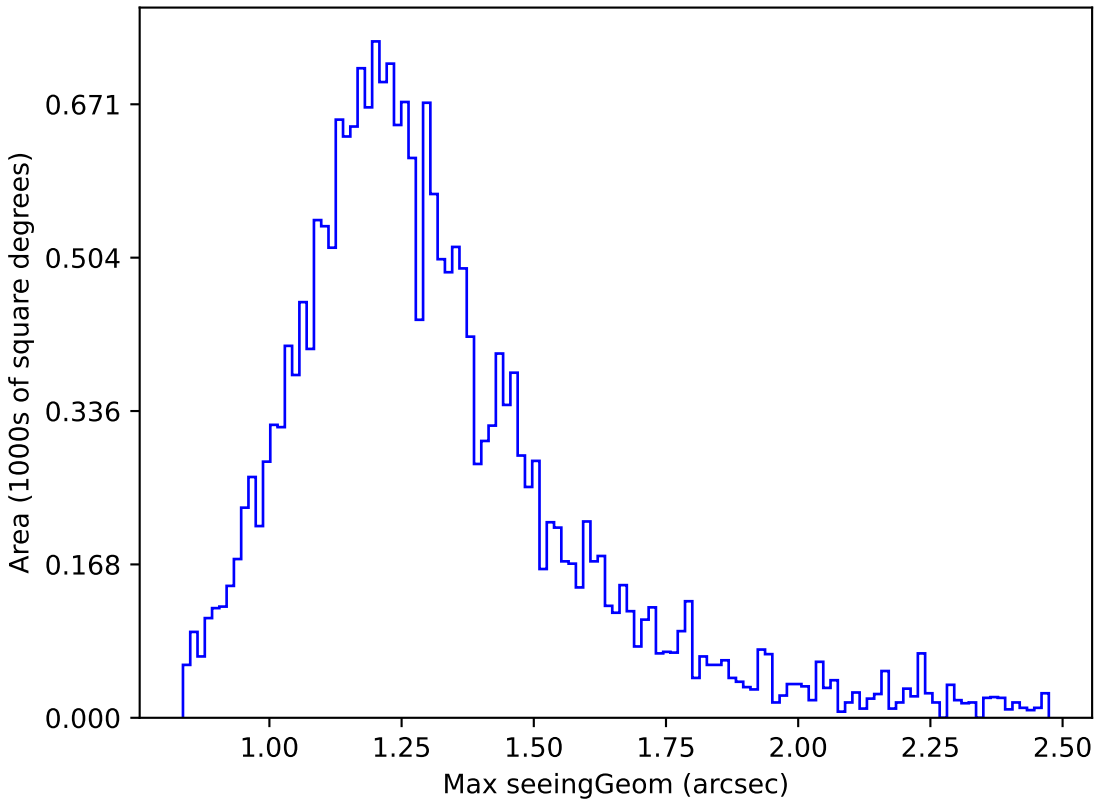
ddf_acor_sf20_lsf0_lsr0_v3.4_10yrs Yr 1 y band: Max seeingGeom
