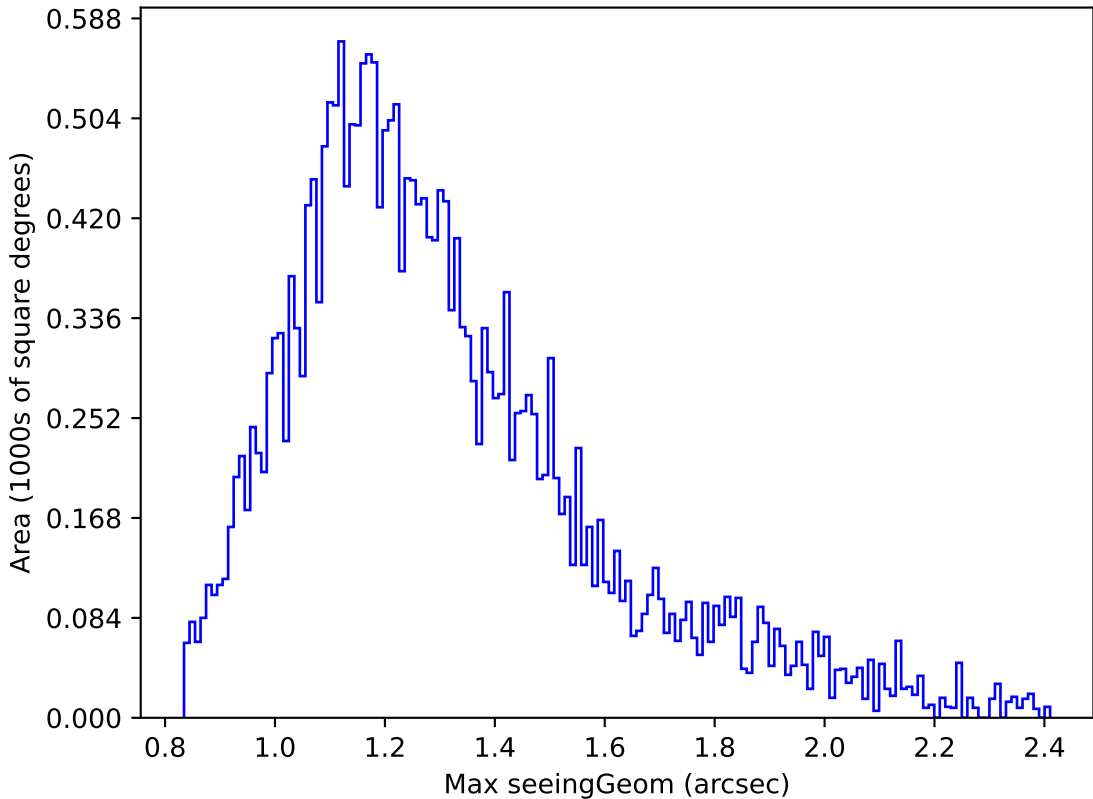
ddf_acor_sf20_lsf0_lsr0_v3.4_10yrs Yr 1 g band: Max seeingGeom
