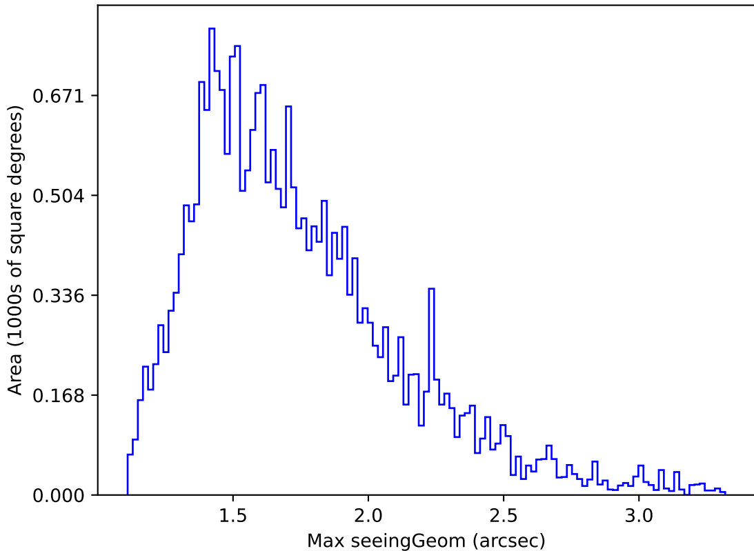
ddf_acor_sf20_lsf0_lsr0_v3.4_10yrs Yr 1 all bands: Max seeingGeom
