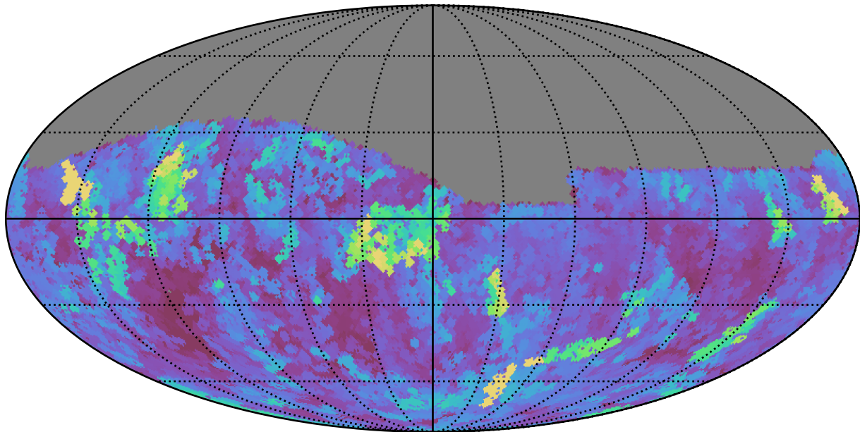
ddf_acor_sf20_lsf0_lsr0_v3.4_10yrs Yr 1 z band: Max seeingEff
