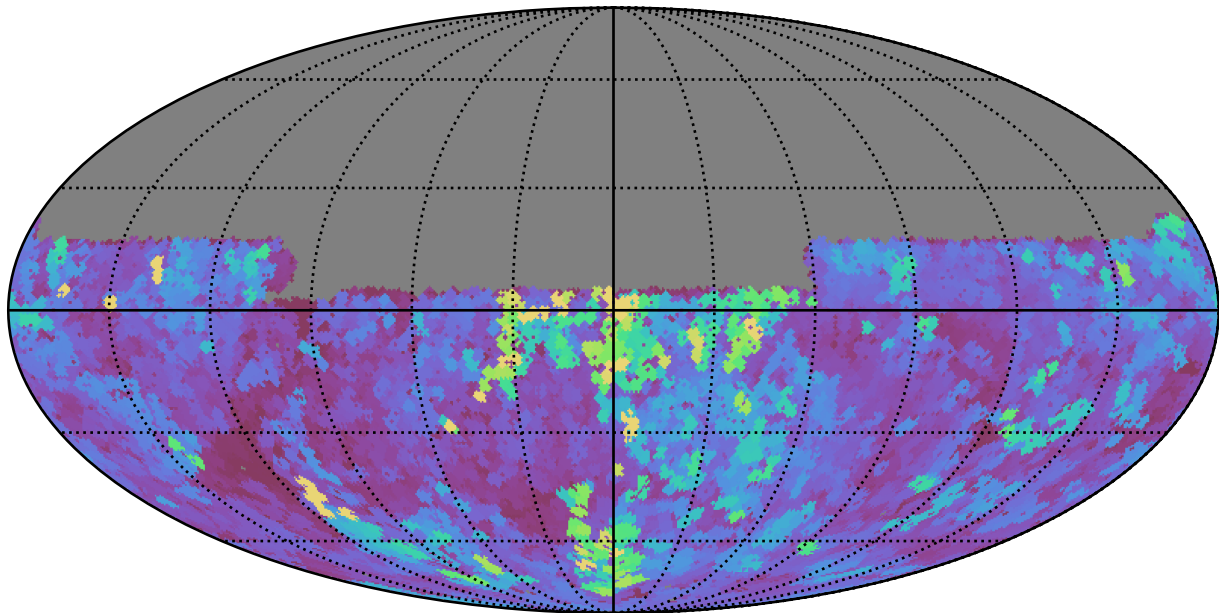
ddf_acor_sf20_lsf0_lsr0_v3.4_10yrs Yr 1 y band: Max seeingEff
