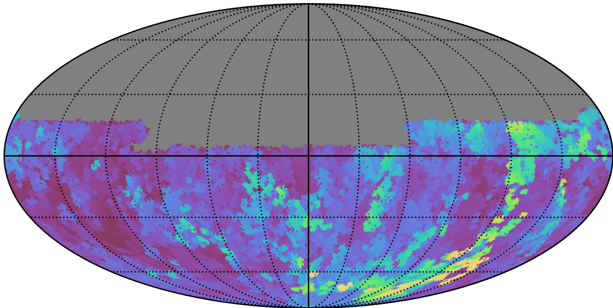
ddf_acor_sf20_lsf0_lsr0_v3.4_10yrs Yr 1 u band: Max seeingEff
