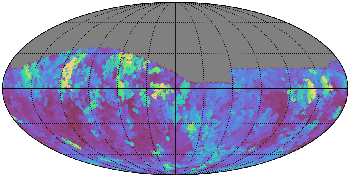
ddf_acor_sf20_lsf0_lsr0_v3.4_10yrs Yr 1 i band: Max seeingEff
