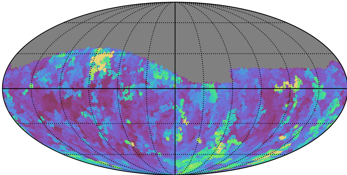
ddf_acor_sf20_lsf0_lsr0_v3.4_10yrs Yr 1 g band: Max seeingEff
