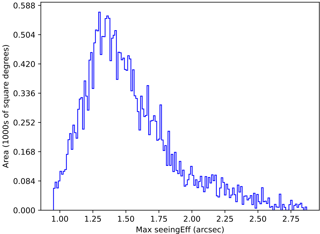
ddf_acor_sf20_lsf0_lsr0_v3.4_10yrs Yr 1 g band: Max seeingEff
