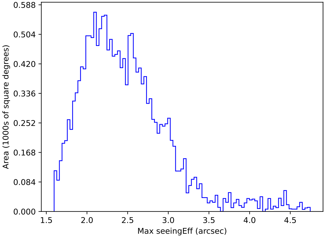
ddf_acor_sf20_lsf0_lsr0_v3.4_10yrs WFD y band: Max seeingEff
