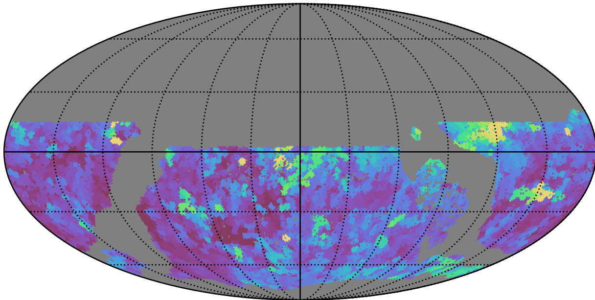
ddf_acor_sf20_lsf0_lsr0_v3.4_10yrs WFD r band: Max seeingEff
