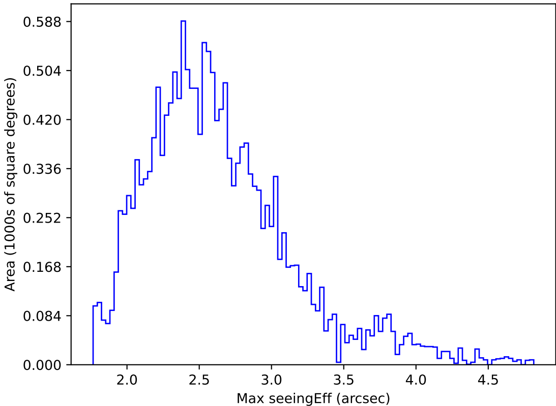
ddf_acor_sf20_lsf0_lsr0_v3.4_10yrs WFD r band: Max seeingEff
