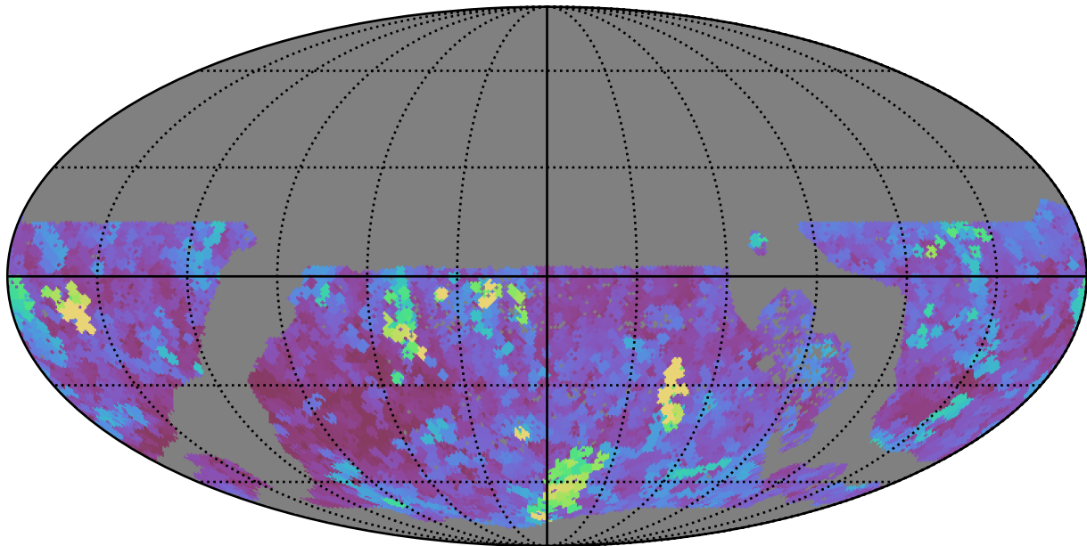
ddf_acor_sf20_lsf0_lsr0_v3.4_10yrs WFD i band: Max seeingEff
