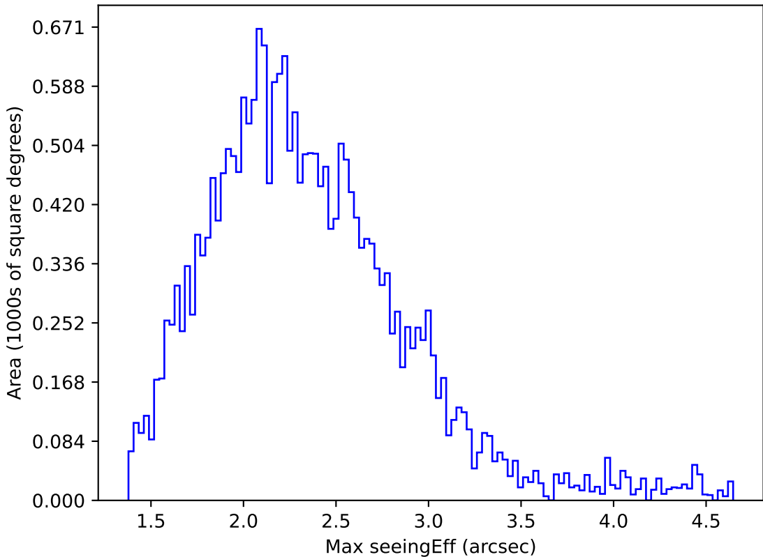
ddf_acor_sf20_lsf0_lsr0_v3.4_10yrs All sky y band: Max seeingEff
