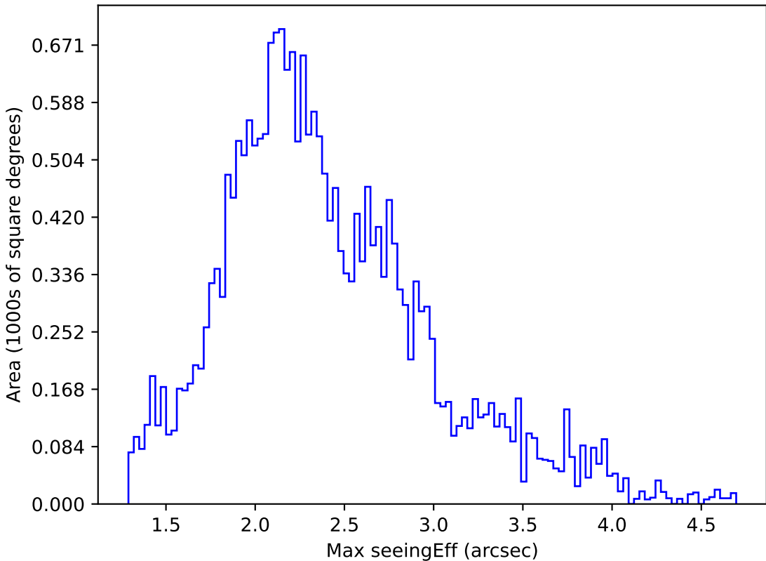
ddf_acor_sf20_lsf0_lsr0_v3.4_10yrs All sky u band: Max seeingEff
