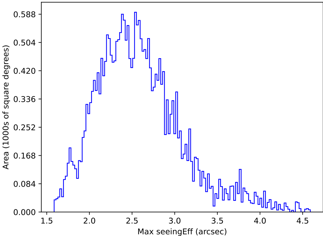
ddf_acor_sf20_ls0_lsr0_v3.4_10yrs All sky r band: Max seeingEff
