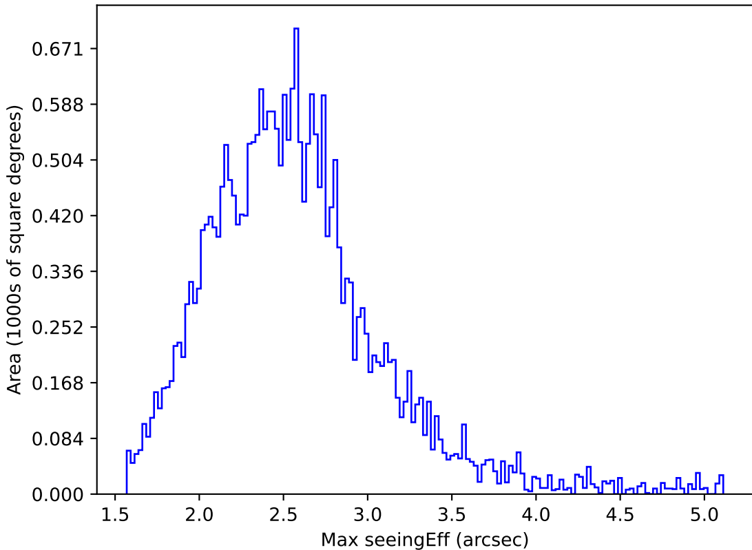
ddf_acor_sf20_ls0_lsr0_v3.4_10yrs All sky i band: Max seeingEff
