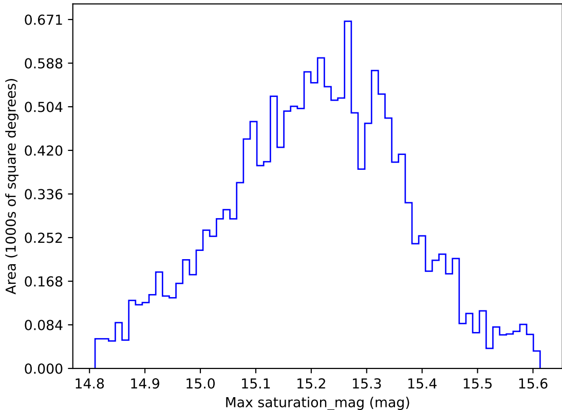
ddf_acor_sf20_lsf0_lsr0_v3.4_10yrs WFD z band: Max saturation_mag
