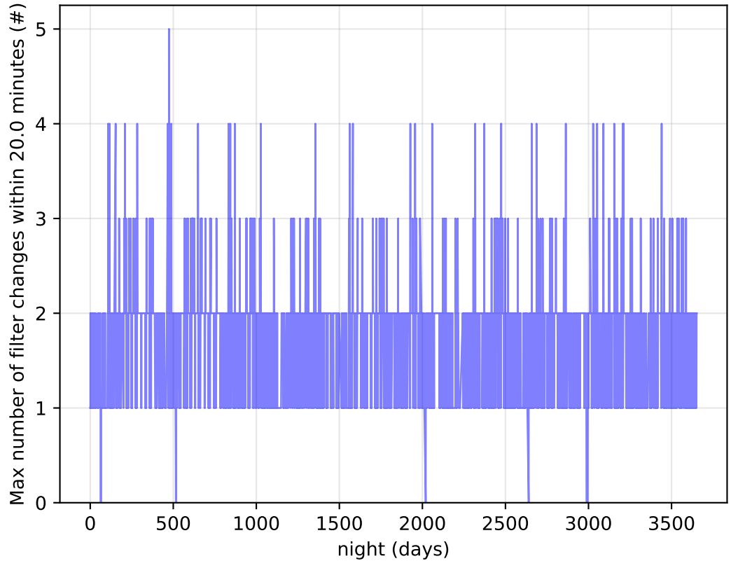
ddf_acor_sf20_lsf0_lsr0_v3.4_10yrs Per Night: Max number of filter changes within 20.0 minutes
