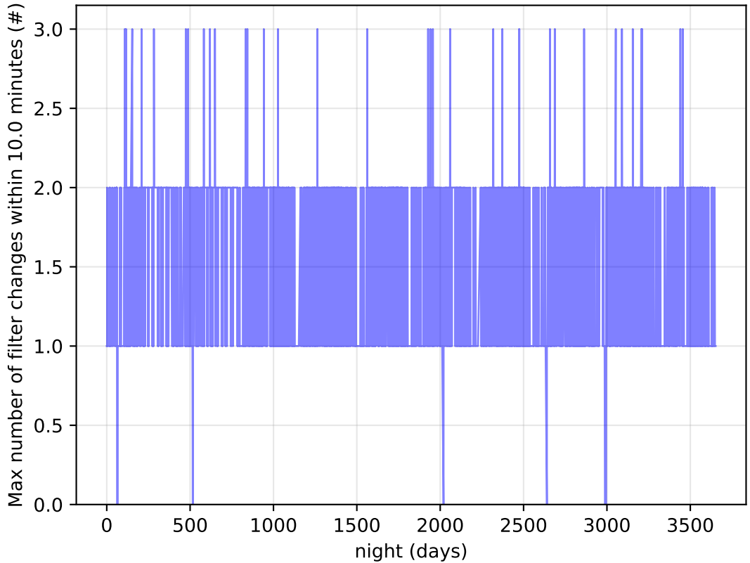
ddf_acor_sf20_Isf0_Isr0_v3.4_10yrs Per Night: Max number of filter changes within 10.0 minutes
