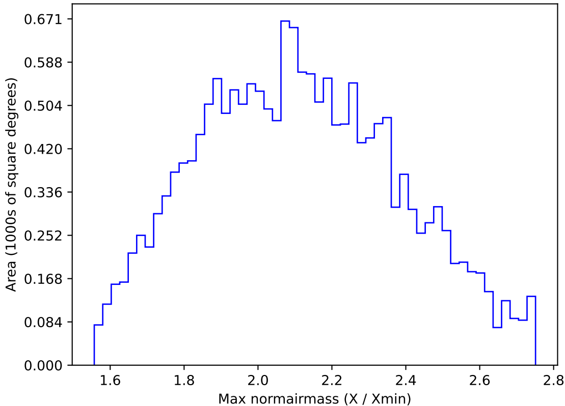
ddf_acor_sf20_lsf0_lsr0_v3.4_10yrs WFD y band: Max normairmass
