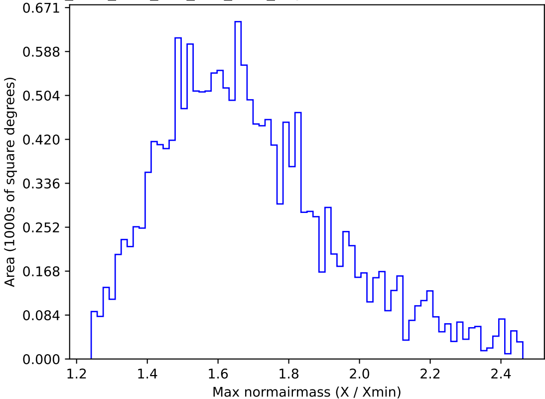
ddf_acor_sf20_lsf0_lsr0_v3.4_10yrs WFD u band: Max normairmass
