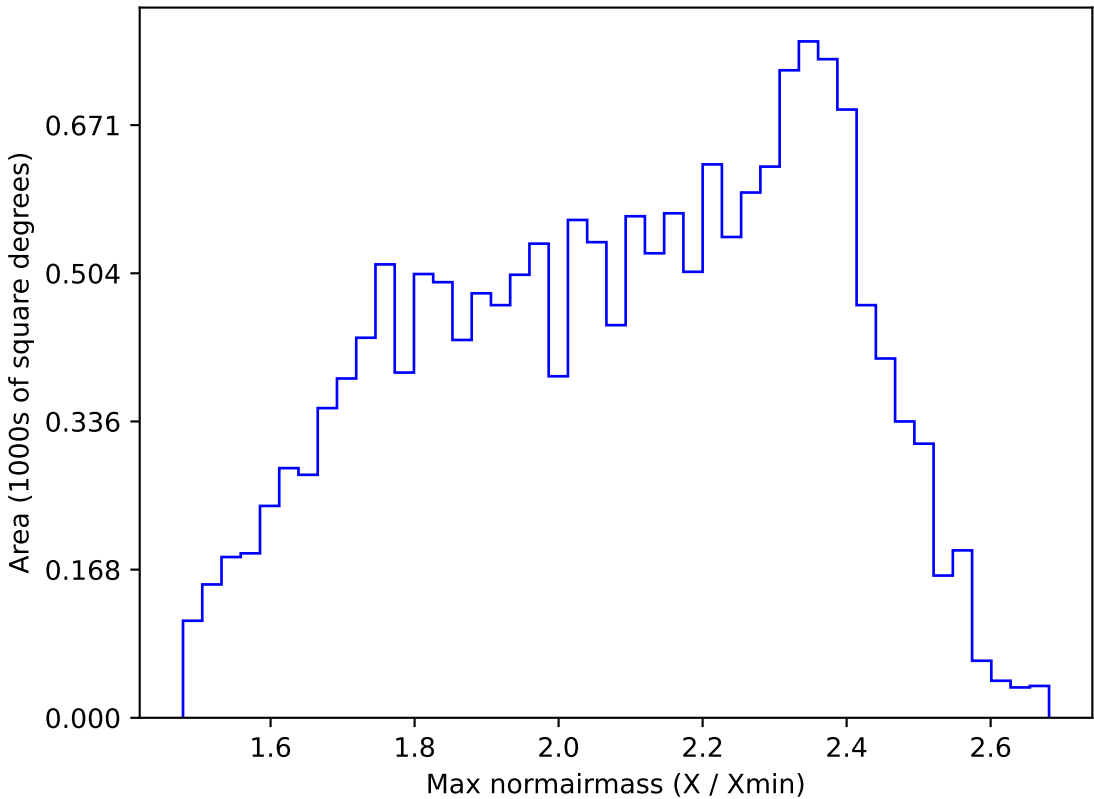
ddf_acor_sf20_lsf0_lsr0_v3.4_10yrs WFD r band: Max normairmass
