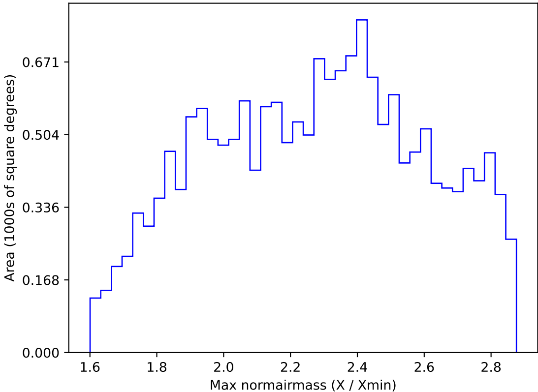
ddf_acor_sf20_lsf0_lsr0_v3.4_10yrs WFD i band: Max normairmass
