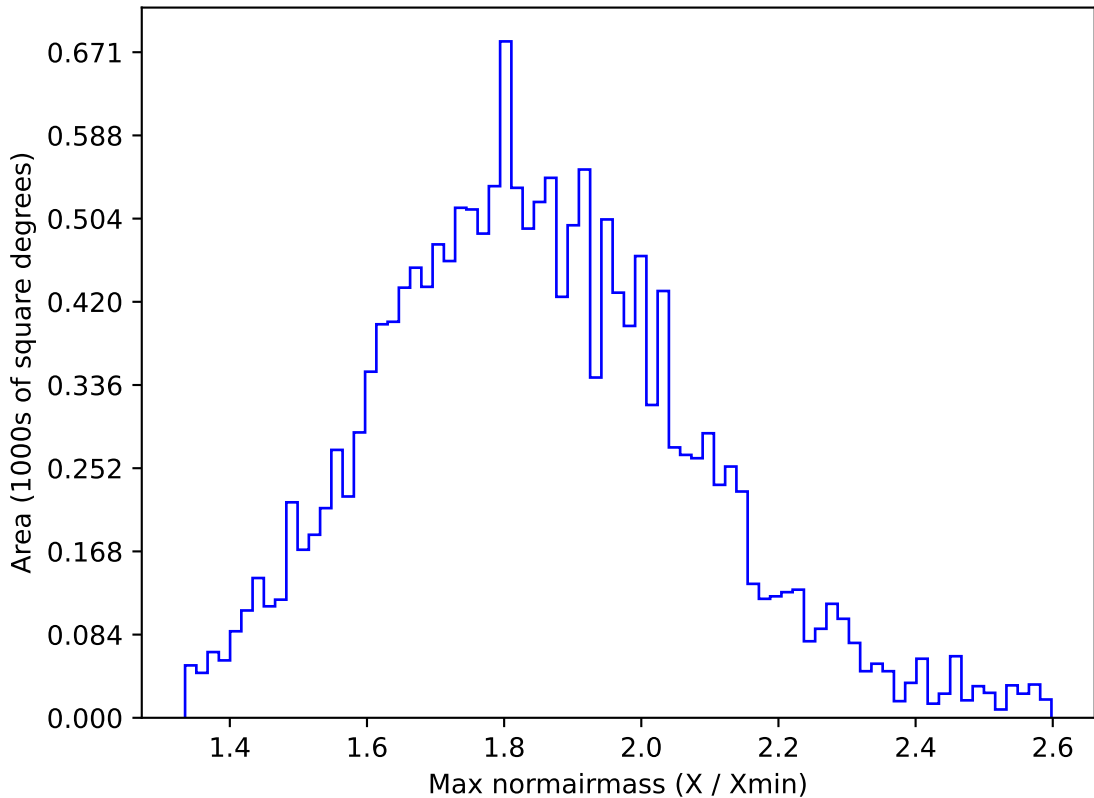
ddf_acor_sf20_lsf0_lsr0_v3.4_10yrs WFD g band: Max normairmass
