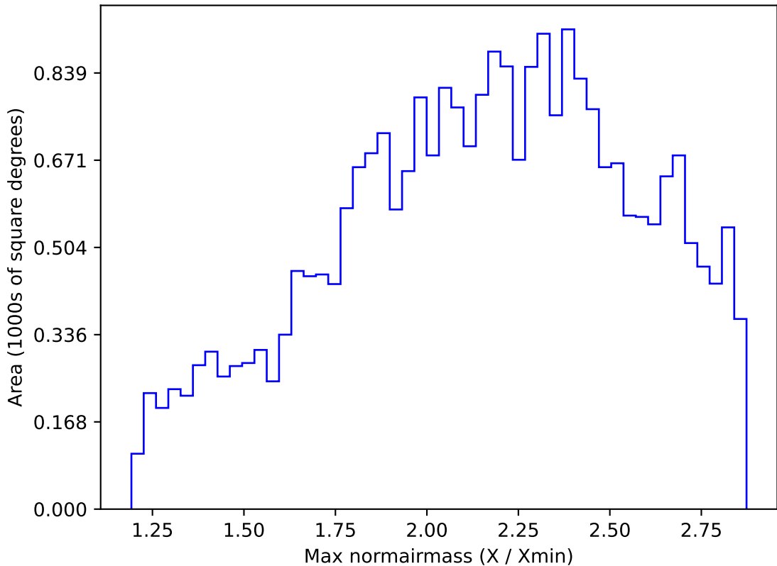
ddf_acor_sf20_lsf0_lsr0_v3.4_10yrs All sky z band: Max normairmass
