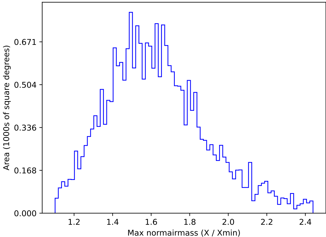
ddf_acor_sf20_lsf0_lsr0_v3.4_10yrs All sky u band: Max normairmass
