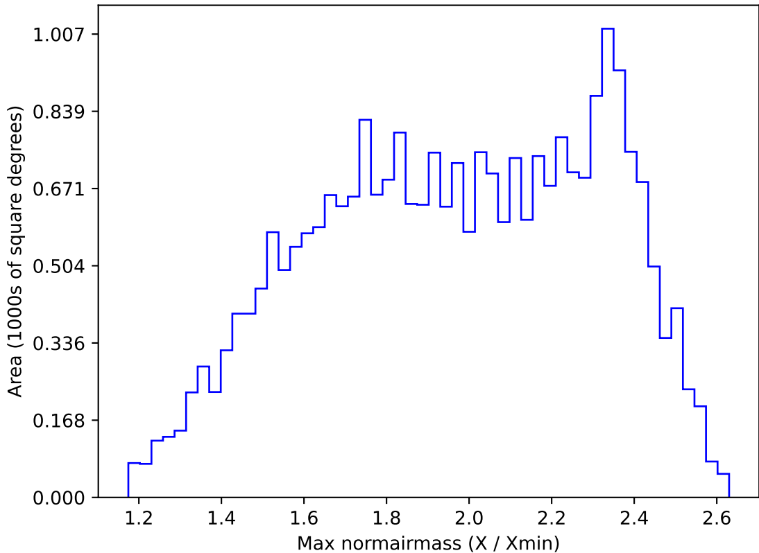
ddf_acor_sf20_lsf0_lsr0_v3.4_10yrs All sky r band: Max normairmass
