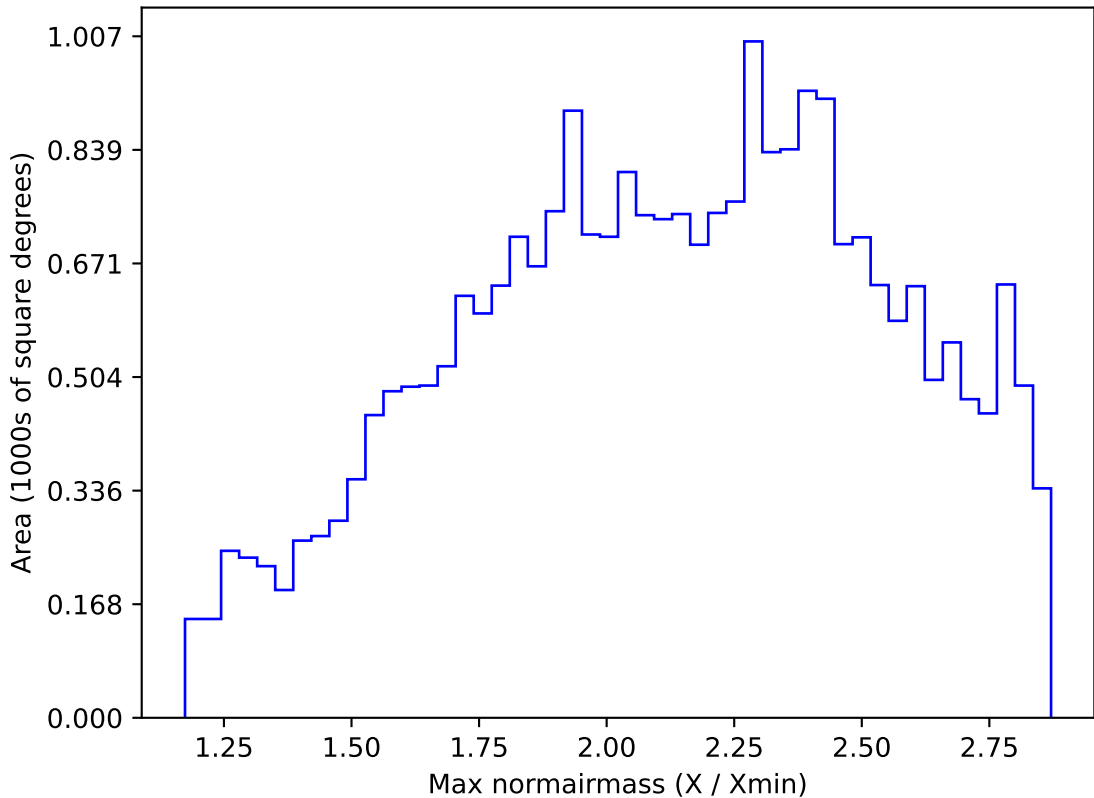
ddf_acor_sf20_lsf0_lsr0_v3.4_10yrs All sky i band: Max normairmass
