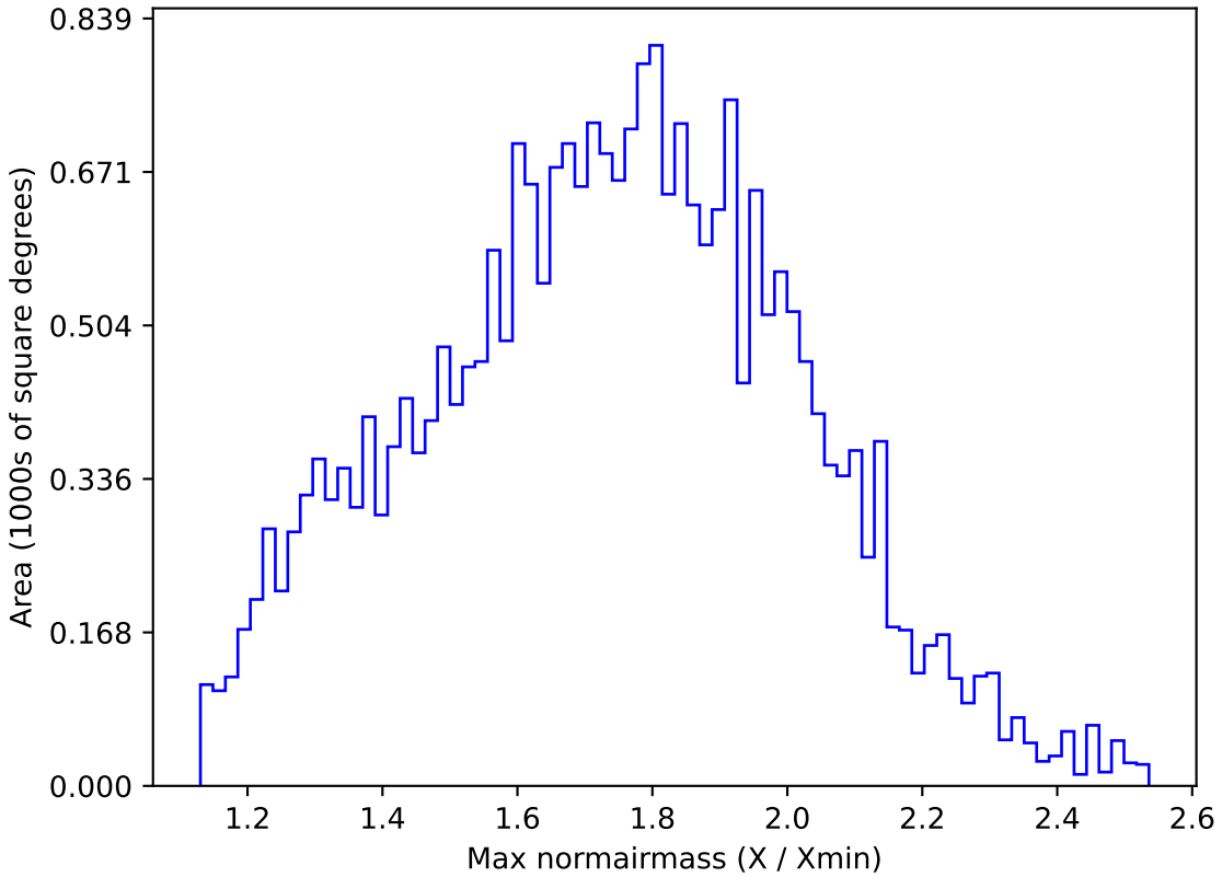
ddf_acor_sf20_lsf0_lsr0_v3.4_10yrs All sky g band: Max normairmass
