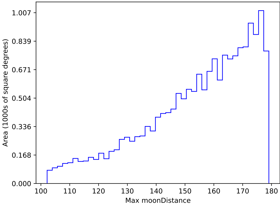
ddf_acor_sf20_lsf0_lsr0_v3.4_10yrs WFD u band: Max moonDistance
