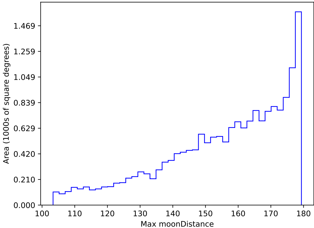
ddf_acor_sf20_lsf0_lsr0_v3.4_10yrs WFD r band: Max moonDistance
