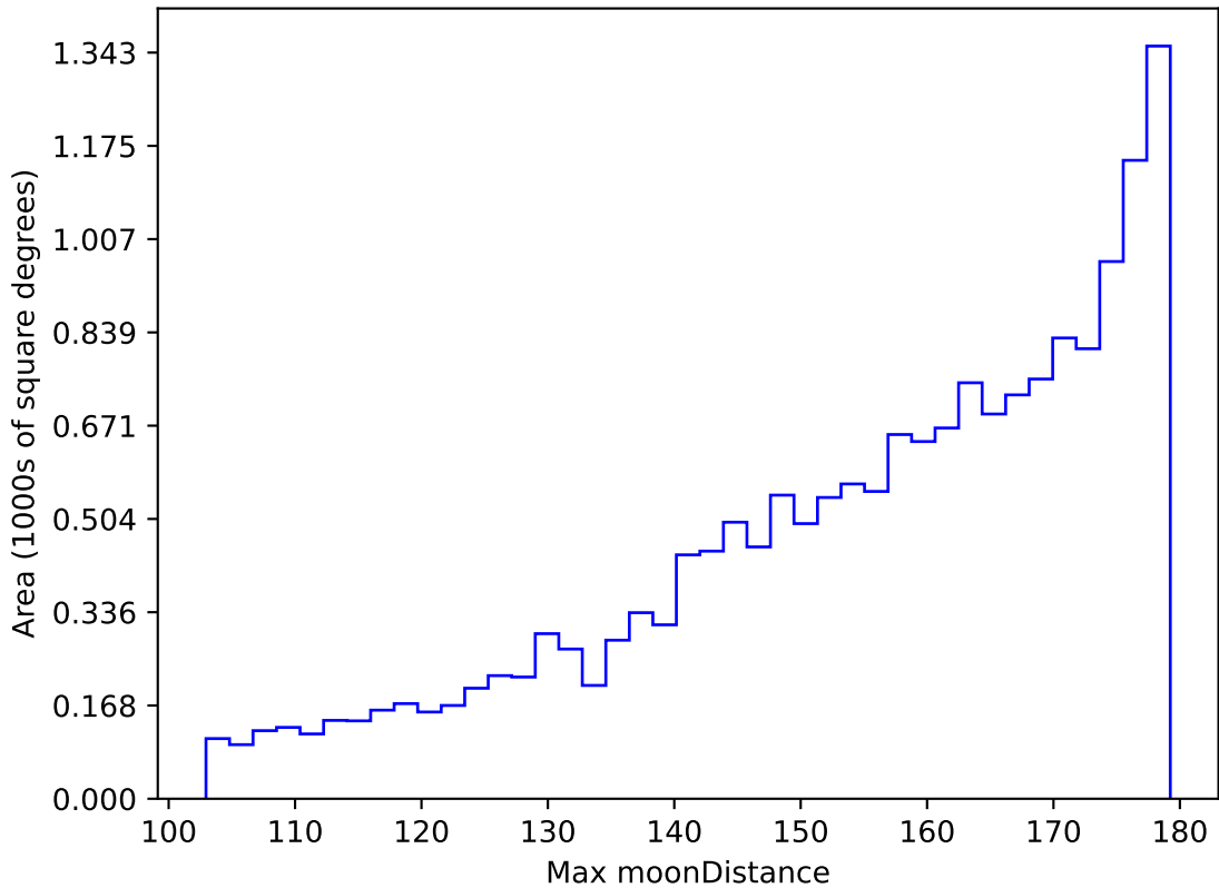
ddf_acor_sf20_lsf0_lsr0_v3.4_10yrs WFD i band: Max moonDistance
