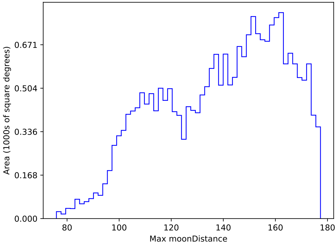
ddf_acor_sf20_lsf0_lsr0_v3.4_10yrs All sky y band: Max moonDistance
