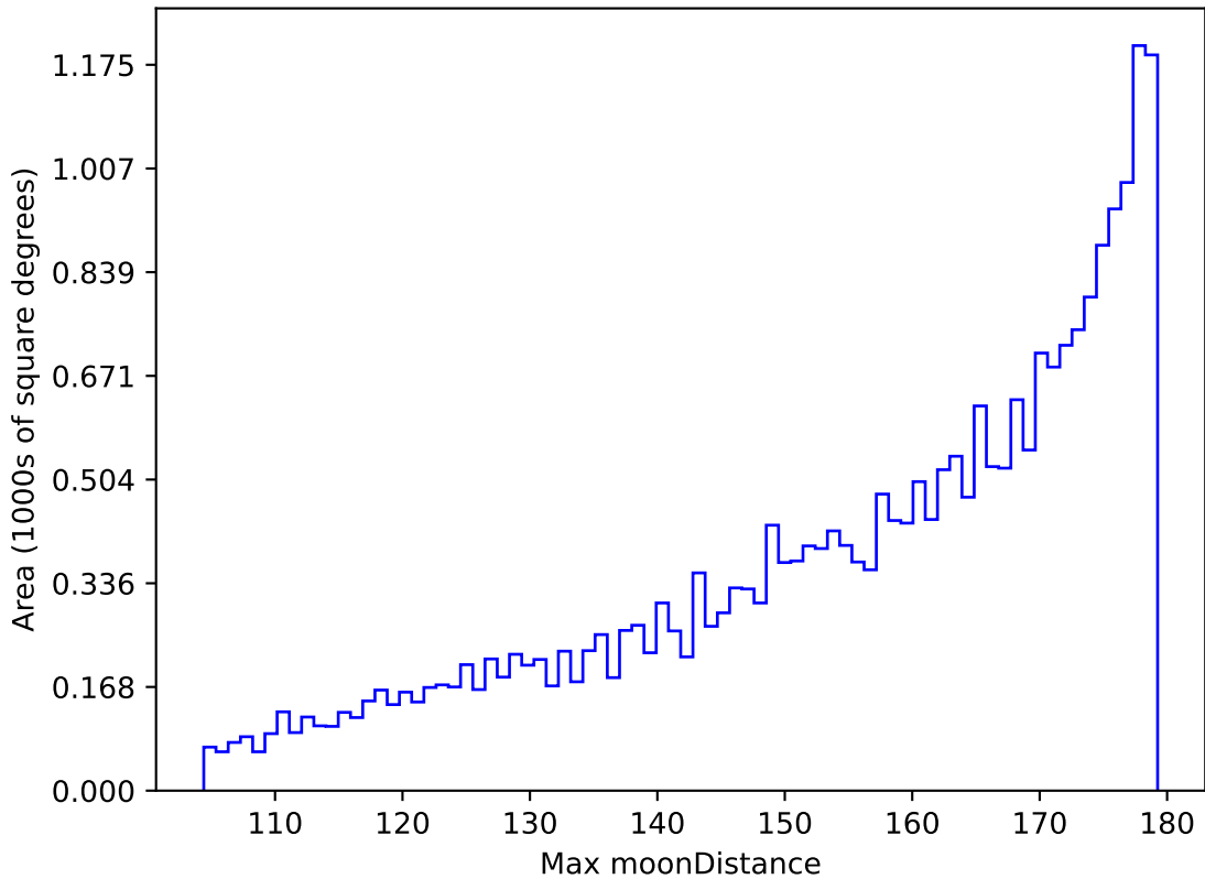
ddf_acor_sf20_lsf0_lsr0_v3.4_10yrs All sky r band: Max moonDistance
