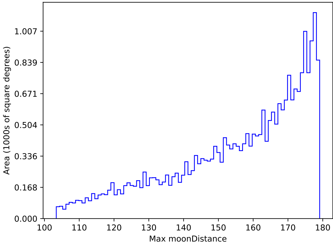
ddf_acor_sf20_lsf0_lsr0_v3.4_10yrs All sky i band: Max moonDistance
