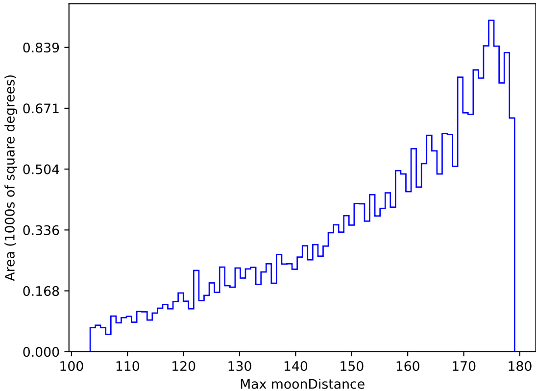
ddf_acor_sf20_lsf0_lsr0_v3.4_10yrs All sky g band: Max moonDistance
